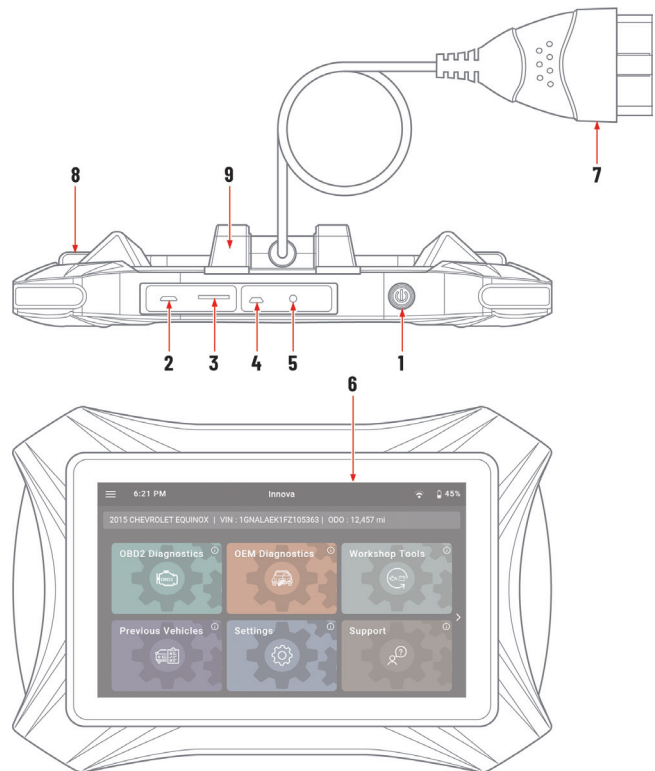
Figure 1: Tablet Controls
